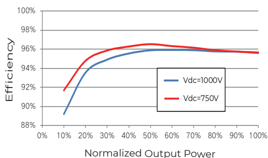
EFFICIENCY CURVE
