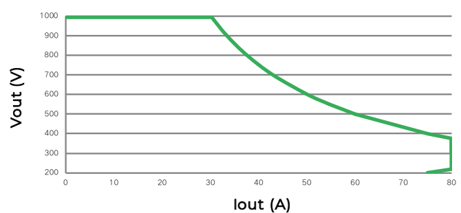
VOUT-IOUT CURVE
